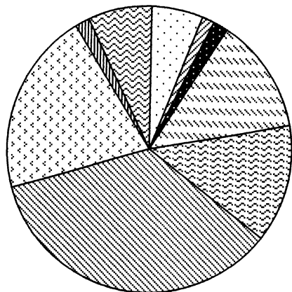
图3 人字洞哺乳动物群中不同门类所占百分比 Composition of the mammalian faunas from Renzidong Cave deposits
